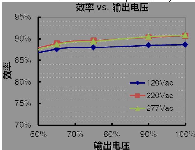
LUD-060S110DS2 (Io=770mA)
