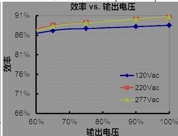
LUD-060S110DS2 (Io=1100mA)
